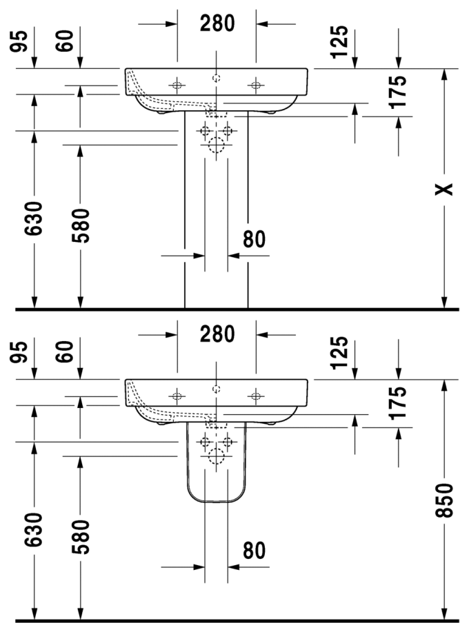
Caption ± Size depending on vanity unit X To determine height please set washbasin on pedestal ↘ In combination with siphon # 0050361000 » Depending on outlet >< Depending on mounting WA Water supply ** Connection tube behind back panel ⚡ Power supply ⌒ P-trap siphon ⌒ Bottle trap siphon
